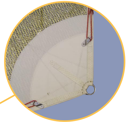
CLEW showing stainless clew ring and alloy leech and foot line cleats.
